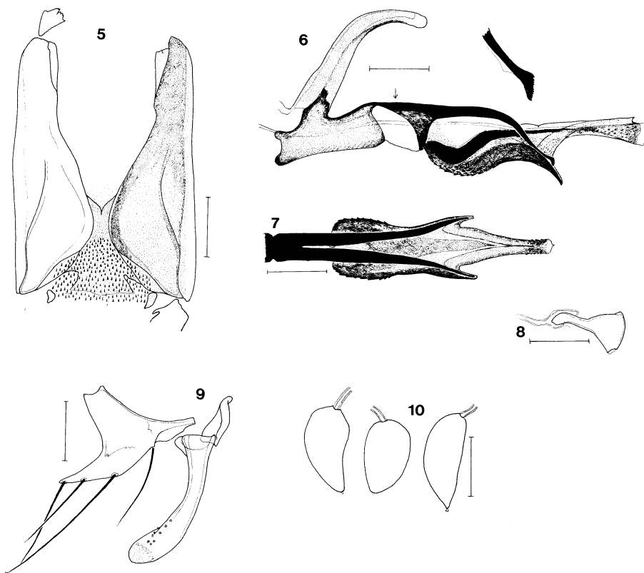
Figs 5–10. Calliphora styliifera (POKORNY). – 5: Bacilliform sclerites and vestiture on membrane between them. – 6: Aedeagus, left lateral view. Inset: tip of paraphallus (enlarged). – 7: Distiphallus, dorsal view. – 8: Ejaculatory sclerite. – 9: Left pre- and postgonites. (Note that the right pregonite of the figured specimen has four distal setae apart from the basal one). – 10: Spermathecae. G. pr. 353. Scales = 0.2 mm.
