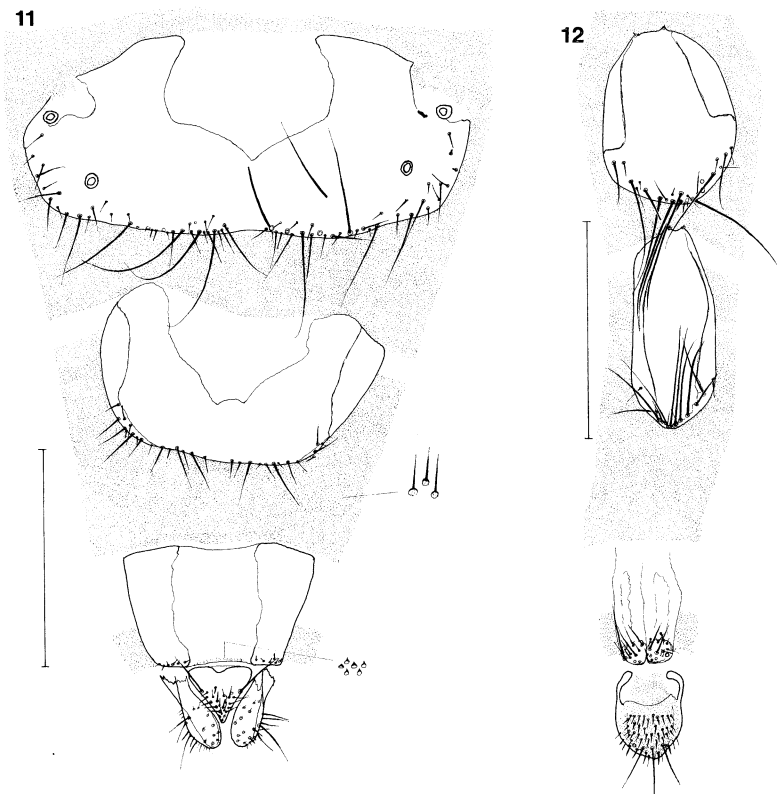
Figs 11–12. Calliphora styliifera (POKORNY), ♀. – 11: Ovipositor, dorsal sclerites. Stipple indicates extent of microtrichiae. Insets: shape of individual microtrichiae in areas indicated. G. pr. 353. – 12: Calliphora styliifera (POKORNY), ♀. Ovipositor, ventral sclerites. Stipple indicates extent of microtrichiae. G. pr. 353. Scales = 1 mm.
